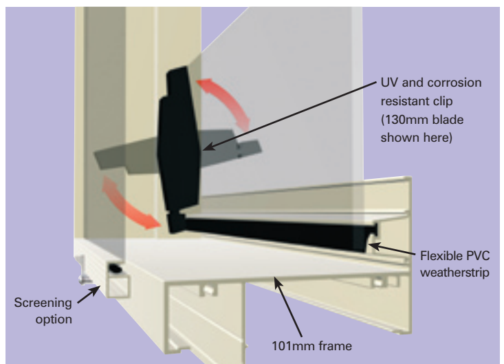
101mm frame / 130mm aluminium blades
