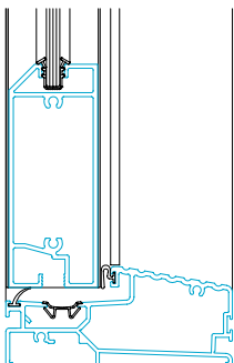
Sill Detail
