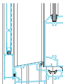
Sill Detail
